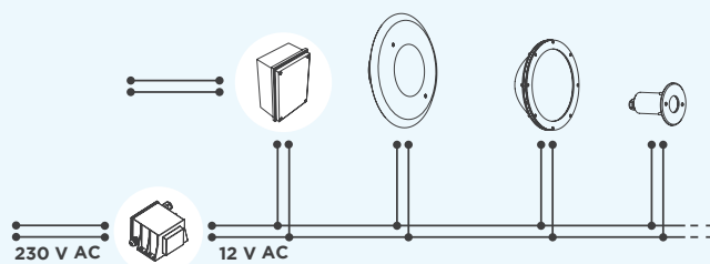
PLC with DMX wiring diagram
