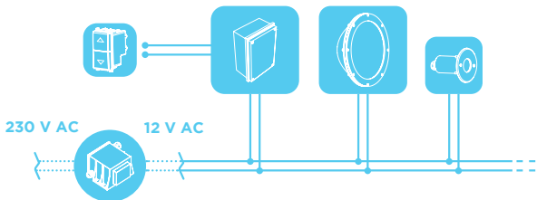
PLC with buttons wiring diagram
